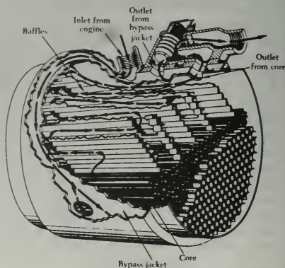
FIGURE 6-5. Oil cooler.
